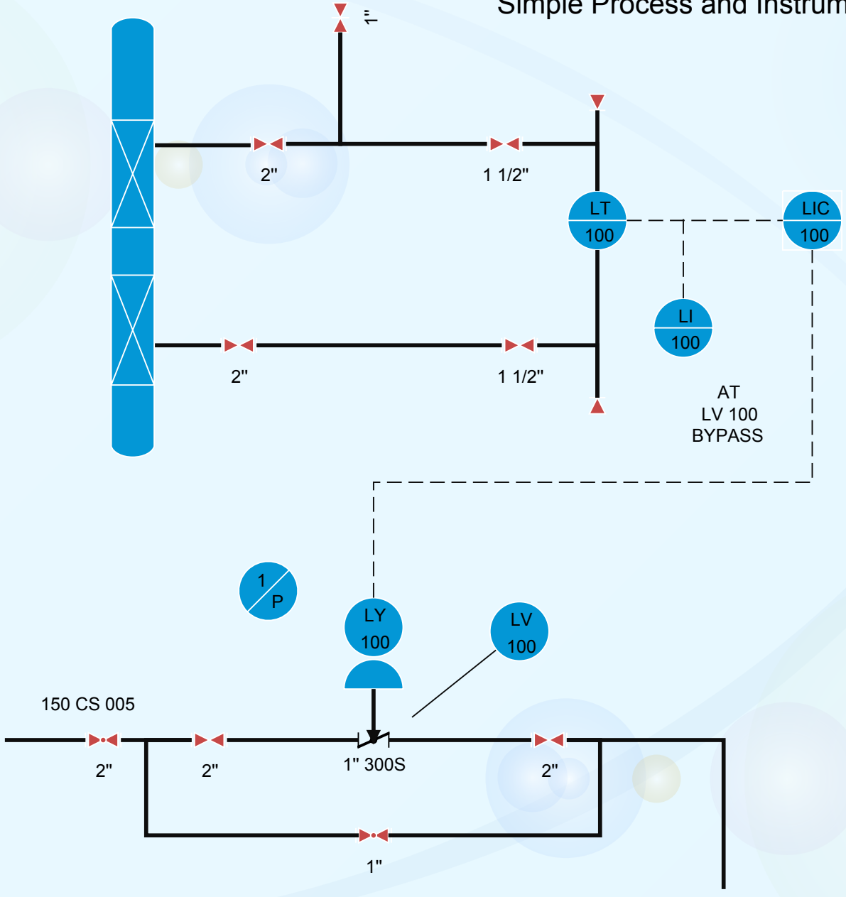
Level Loop LIC-100
